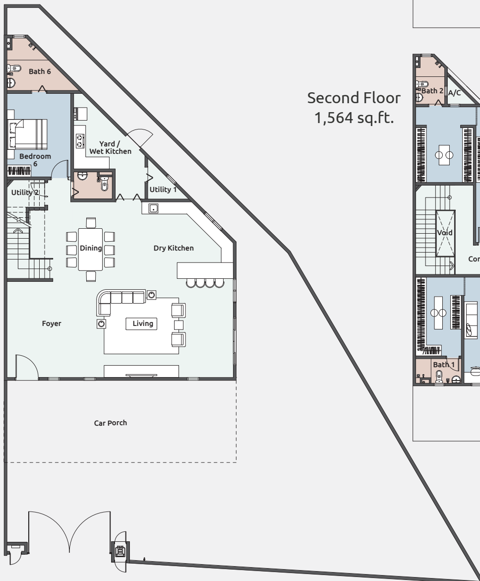
Ground Floor 2,086 sq.ft.
